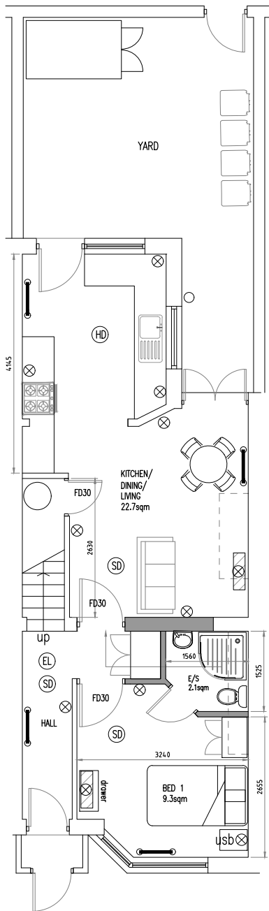
PROPOSED GROUND FLOOR LAYOUT 1:100 @ A3
