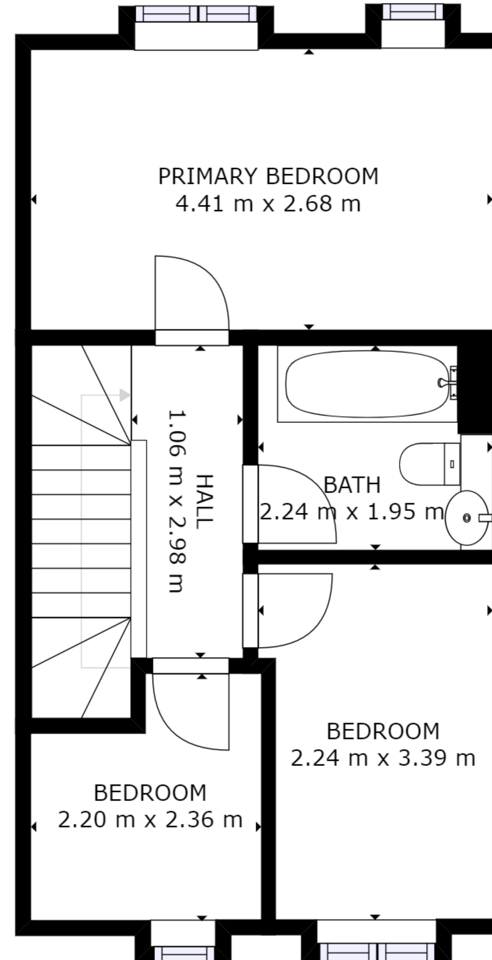
FLOOR 2
